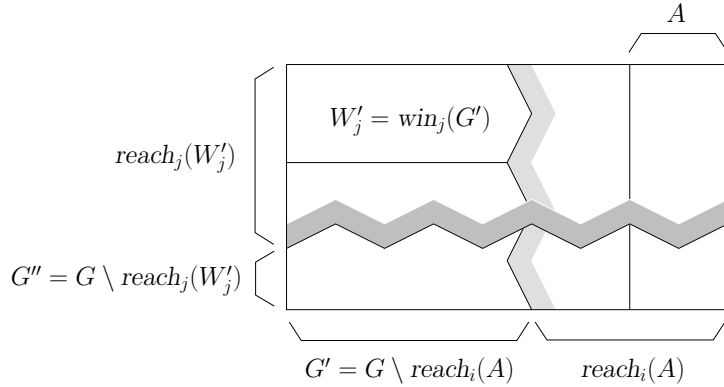
FIG. 5.2. A game G and its subgames G' = G \setminus \mathit{reach}_i(A) and G'' = G \setminus \mathit{reach}_j(W'_j) .
