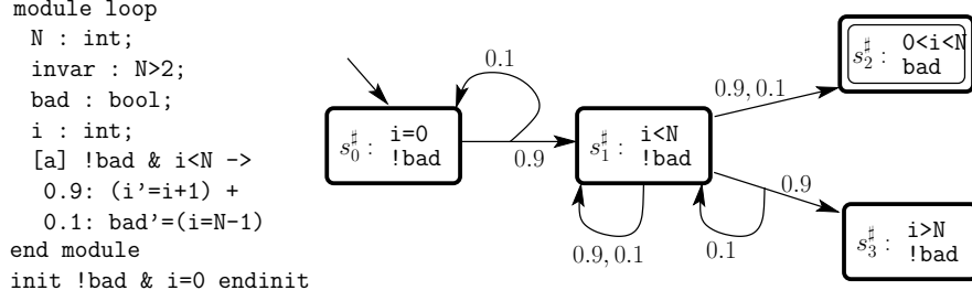
Fig. 2. Cycle program and the quotient automaton with respect to i=0, \text{bad}, i<N
