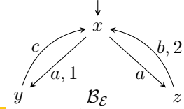
Figure 1 A Büchi automaton.
