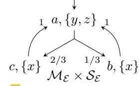
Figure 4 The product of \mathcal{M}_\varepsilon and \mathcal{S}_\varepsilon .
