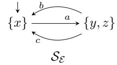
■ Figure 3 The subset construction for \mathcal{B}_\varepsilon .
